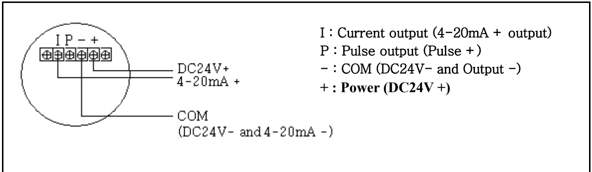
Figure 3-8. VFM 8300 Series wiring Terminal drawing
