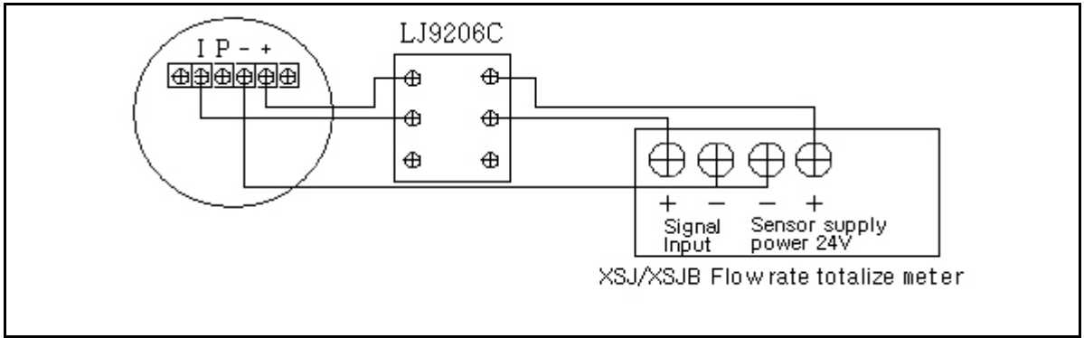
Figure 3-7. VFM 8300 Series Explosion place wiring connection
