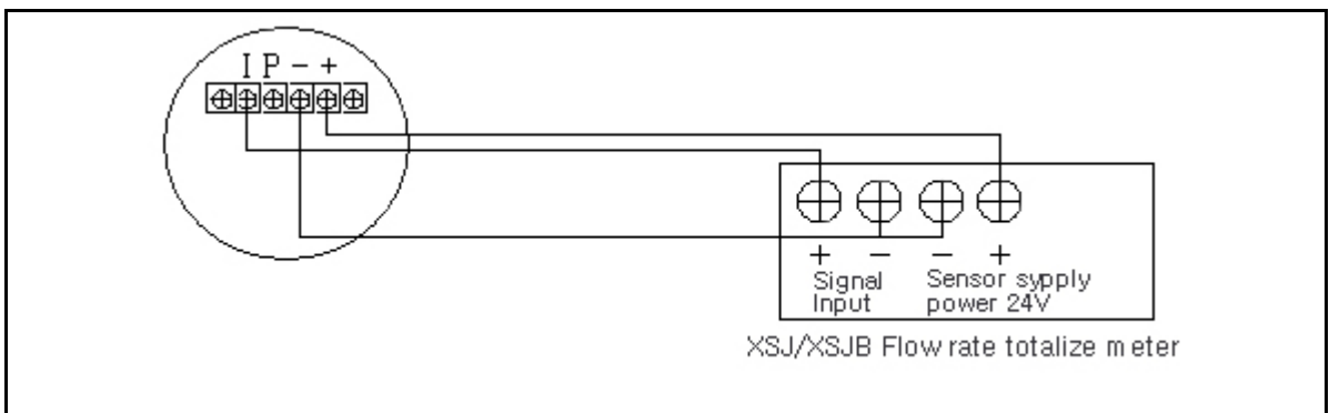
Figure 3-6. VFM 8300 and XSJ/XSJB wiring connection
